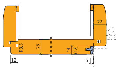
Door lining profile
