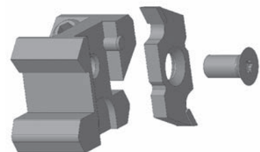
Knife holder to adapt grooving knives.
