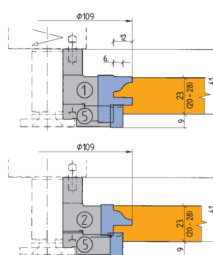
Tongue 6 mm, inserted and beaded panels
