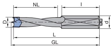
Dowel drill
