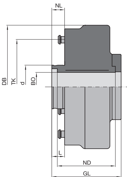
Hydro quick clamping sleeve type 160 HF
