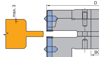
Tongue profile
