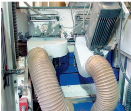
Problem: Machine wear through abrasive chips.
