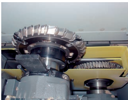
DFC® hogger with shredding edges shred the veneer projection on an extractable size for a complete disposal.
