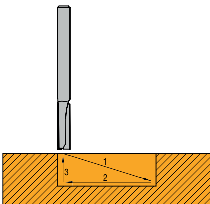
Vertical grooves
