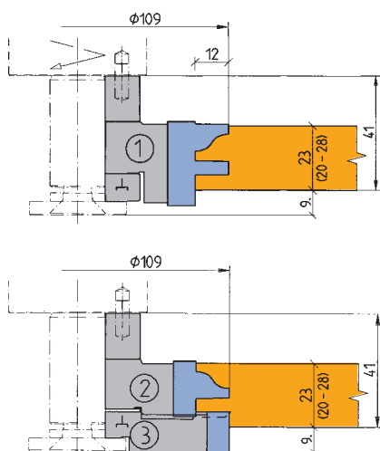
Messing 12 mm, ingeschoven paneel
