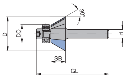
WO 314-1-02; fasefrees 30°
