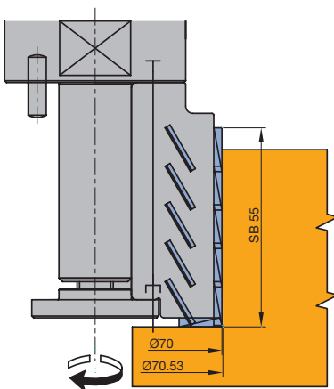
Diamaster WhisperCut sponningmesenkop
